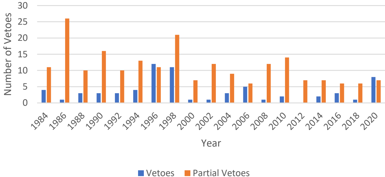
Senate Bill Vetoes and Partial Vetoes, Even Years 1984-2020
